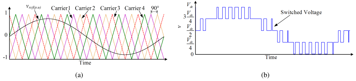
Fig. 2. PS-PWM technique for a five-level converter: (a) reference sinusoidal signal with four triangular carriers and (b) switched phase voltage.
