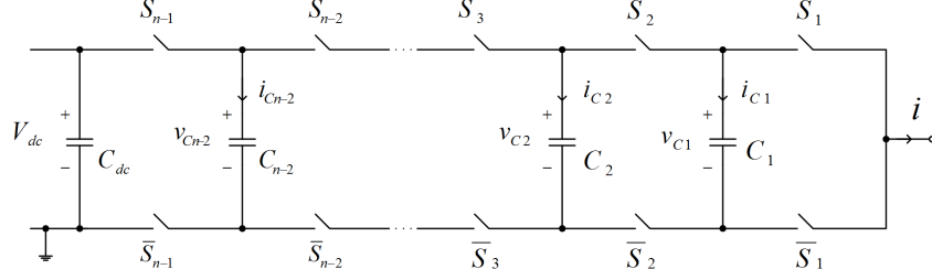
Fig. 1. Phase-leg of an n -level FLC Converter.
