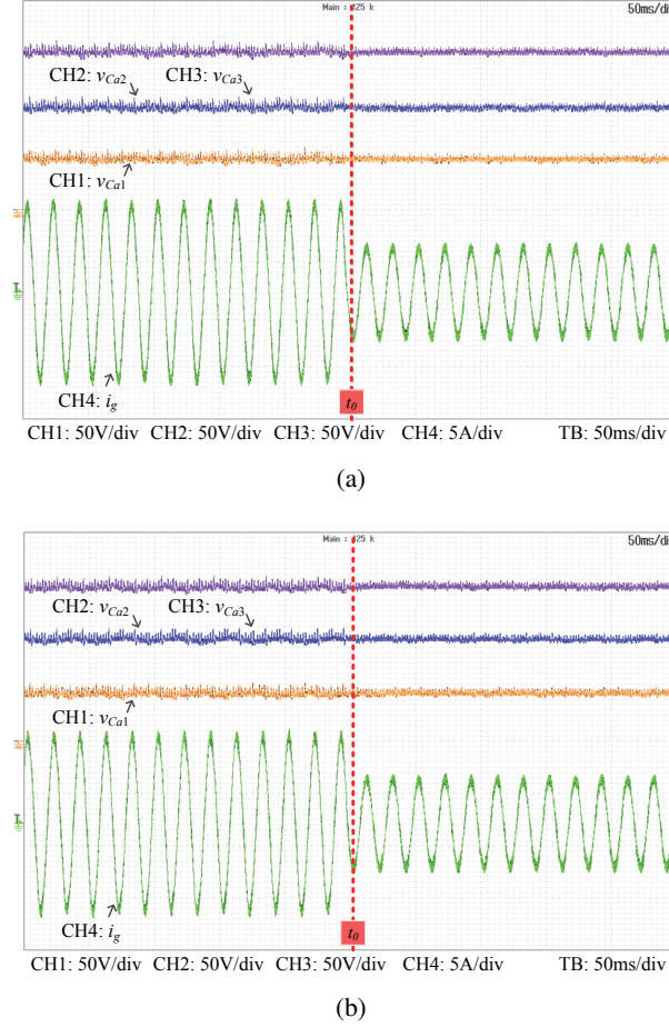
Fig. 10. Comparison of capacitor voltages during a step load change at t_0 : (a) the conventional balancing method in [27] and (b) the proposed balancing method.
