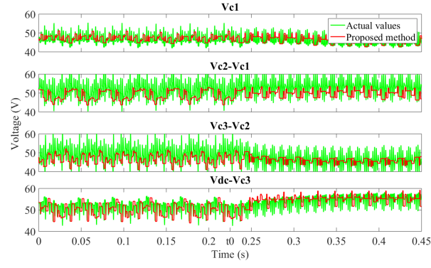
Fig. 11. Measured controllers' feedback signals using the proposed single voltage sensor measurement method and using multiple voltage sensors (actual values) during a step change in the ac reference voltage at t_0 .
