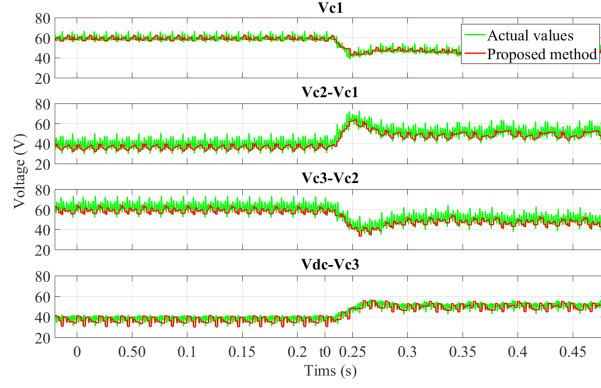
Fig. 7. Measured controllers' feedback signals using the proposed single voltage sensor method and using multiple voltage sensors (actual values) during a sudden balancing method activation test.
