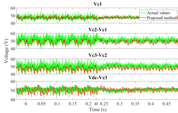
Fig. 9. Measured controllers' feedback signals using the proposed single voltage sensor measurement method and using multiple voltage sensors (actual values) during a step load change at t_0 .
