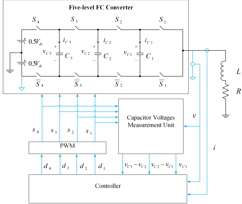
Fig. 6. Circuit diagram of the experimental system.
